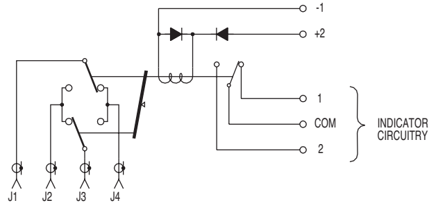
SCHEMATIC SHOWN IN FAILSAFE POSITION
