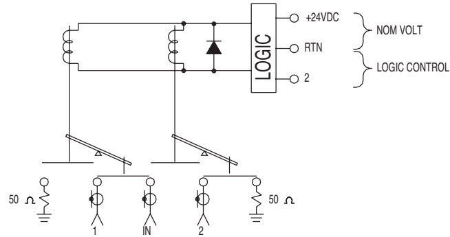
SCHEMATIC SHOWN IN FAILSAFE POSITION
