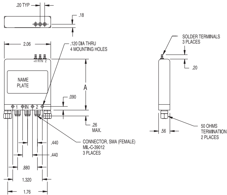
Series 022 Switch with External Terminations
