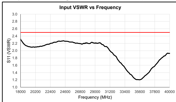
Typical Performance @ 23°C (Reference S/N 2332804) [30 dB Gain, +10 dBm P1dB Model Shown]
