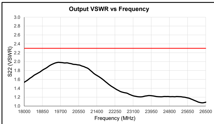
Typical Performance @ 23°C (Reference S/N 2347603) [30 dB Gain, +10 dBm P1dB Model Shown]
