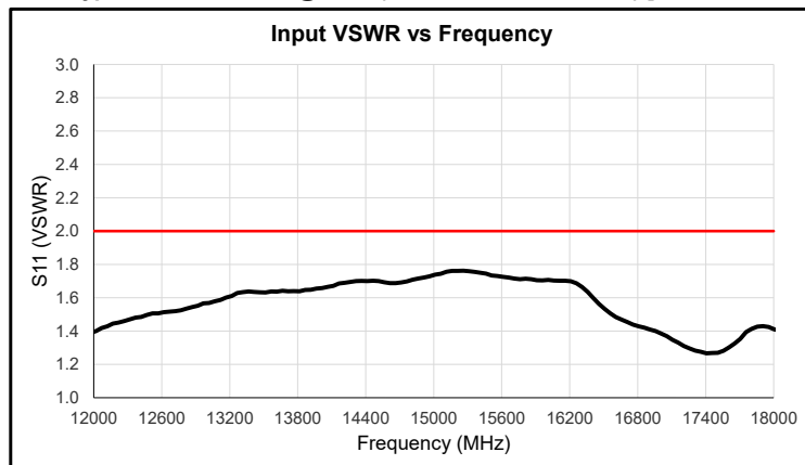
Typical Performance @ 23°C (Reference S/N 2332803) [30 dB Gain, +10 dBm P1dB Model Shown]
