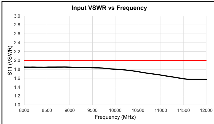
Typical Performance @ 23°C (Reference S/N 2347602) [30 dB Gain, +10 dBm P1dB Model Shown]
