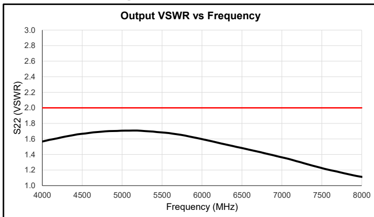
Typical Performance @ 23°C (Reference S/N 2347601) [30 dB Gain, +10 dBm P1dB Model Shown]
