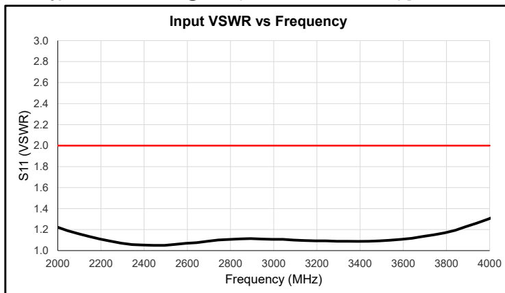
Typical Performance @ 23°C (Reference S/N 2332812) [40 dB Gain, +10 dBm P1dB Model Shown]
