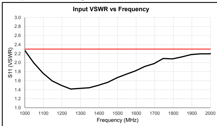
Typical Performance @ 23°C (Reference S/N 2333091) [40 dB Gain, +10 dBm P1dB Model Shown]
