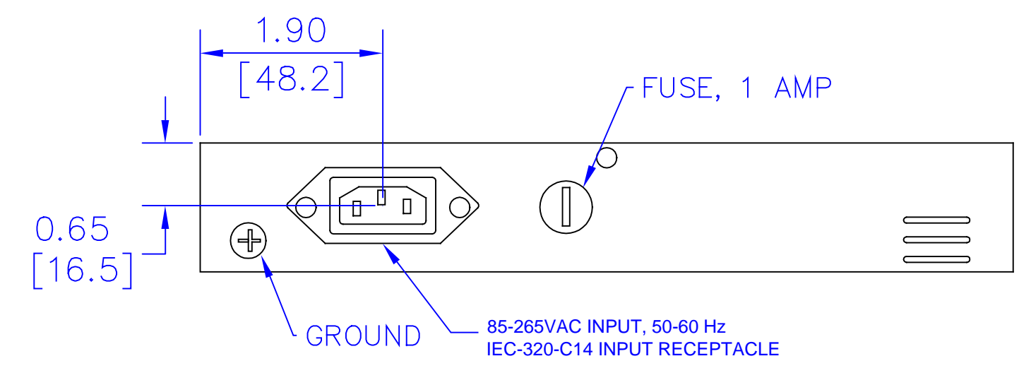
REAR VIEW
