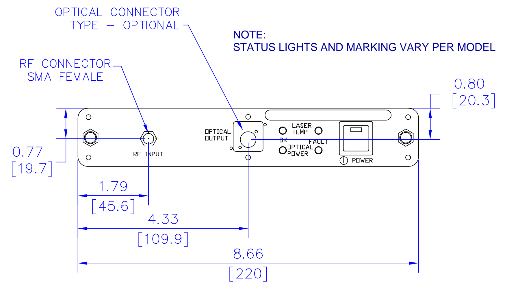
FRONT VIEW
