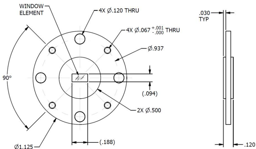
OUTLINE DRAWING - 19-230-6R-6R
