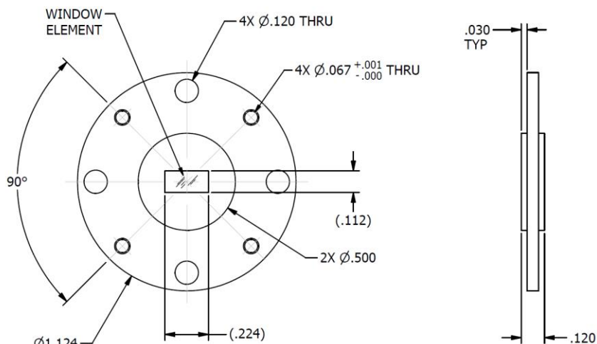
OUTLINE DRAWING - 22-230-6R-6R
